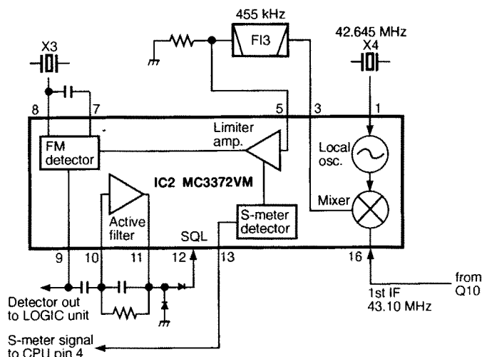
Fig. 1 VHF 2ND IF AMPLIFIER
